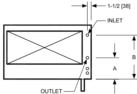
TOP VIEW (FILTER RACK OMITTED) (RIGHT HAND UNIT)
